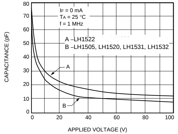
B. Switch Capacitance vs. Applied Voltage
