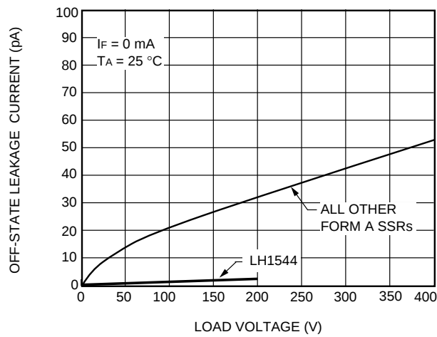
A. Leakage Current vs. Applied Voltage
