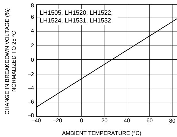
D. Switch Breakdown Voltage vs. Temperature
