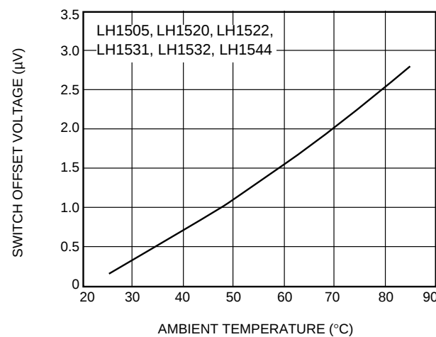
F. Switch Offset Voltage vs. Temperature
