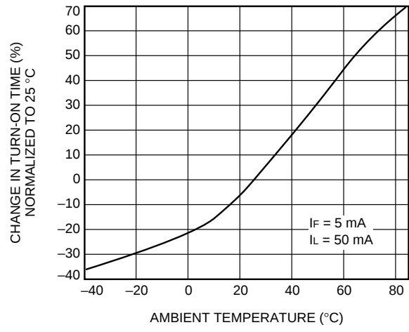
D. Turn-On Time vs. Temperature (LH1544)
