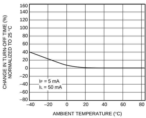
F. Turn-Off Time vs. Temperature (LH1544)
