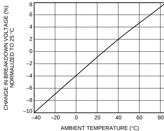
E. Switch Breakdown Voltage vs. Temperature (LH1544)
