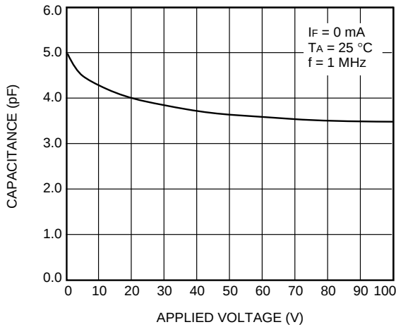
C. Switch Capacitance vs. Applied Voltage (LH1544)
