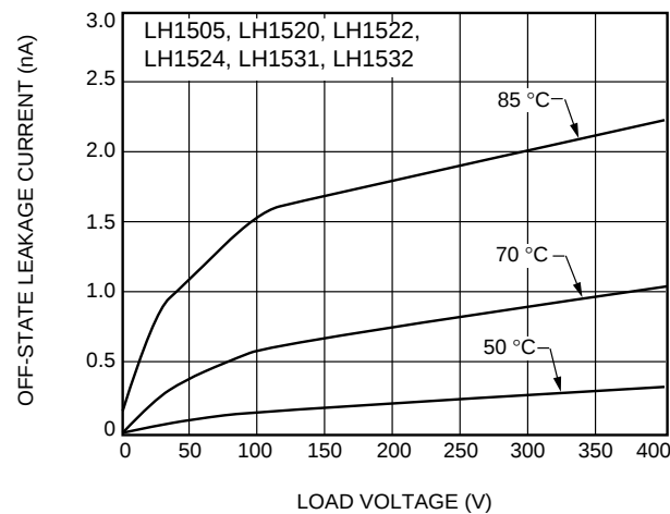
B. Leakage Current vs. Applied Voltage at Elevated Temperatures
