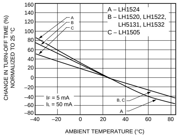
E. Turn-Off Time vs. Temperature
