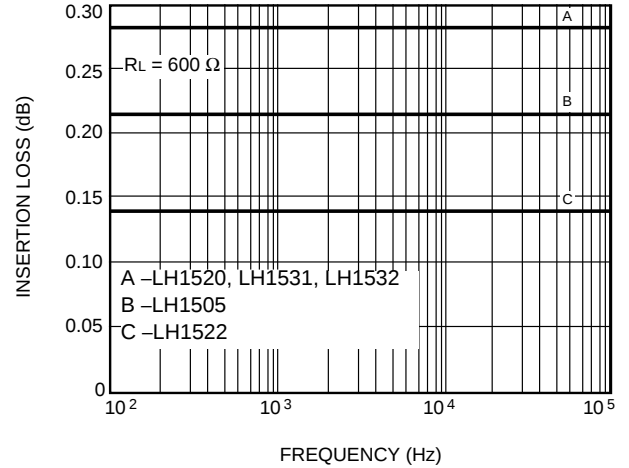
D. Insertion Loss vs. Frequency
