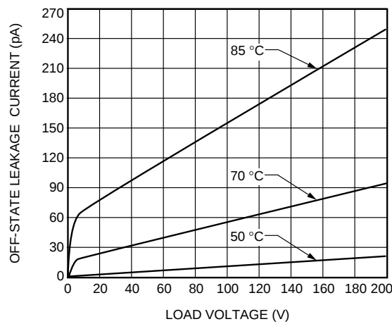
C. Leakage Current vs. Applied Voltage at Elevated Temperatures (LH1544)
