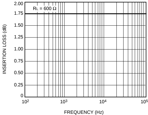
E. Insertion Loss vs. Frequency (LH1544)
