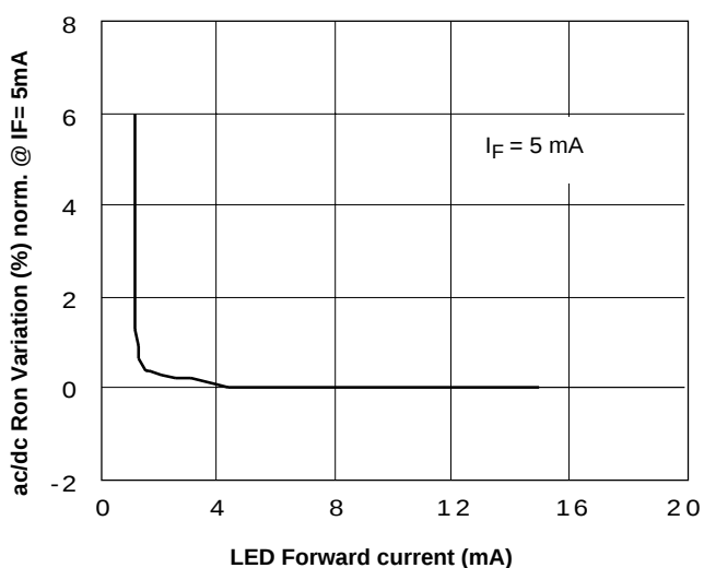
Figure 11. Variation in ON-Resistance vs. LED Current
