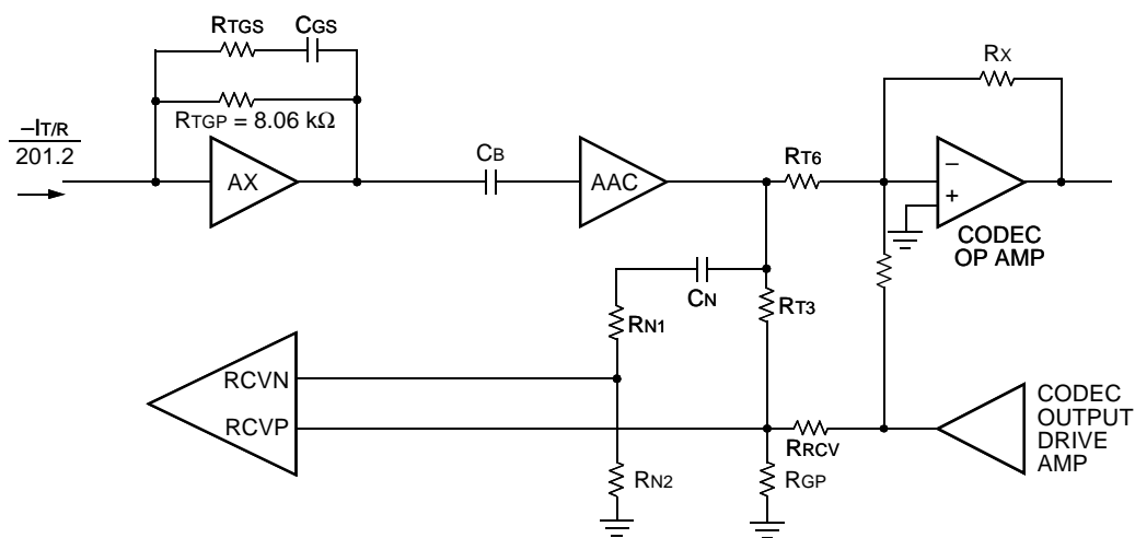
Figure 17. Interface Circuit Using First-Generation Codec ( \pm 5 V Battery)
