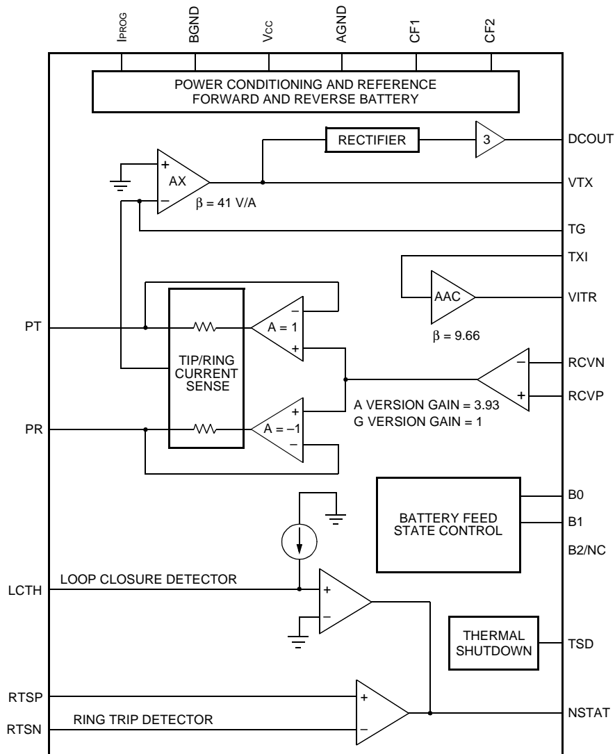
Figure 1. Functional Diagram
