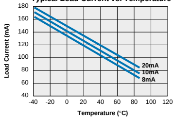
LCC110 - FormA Typical Load Current vs. Temperature
