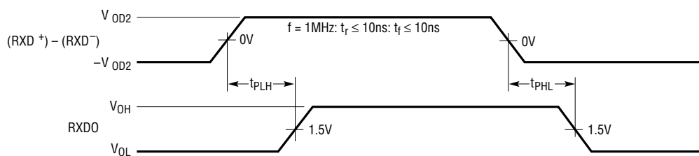
Figure 6. Differential Receiver
