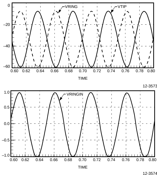
Figure 11. Ring Mode Typical Operation
