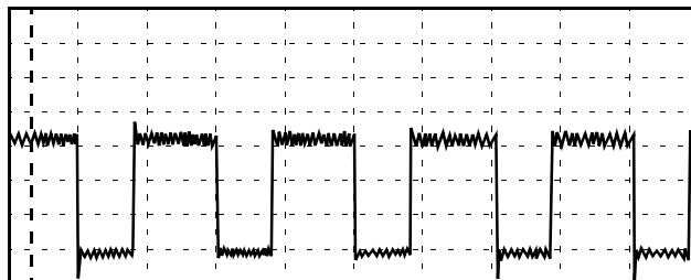
Figure 15. 5 V PWM Signal Amplitude
