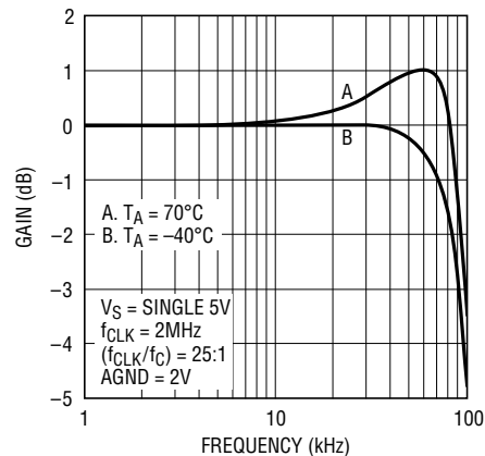
Maximum Passband vs Temperature
