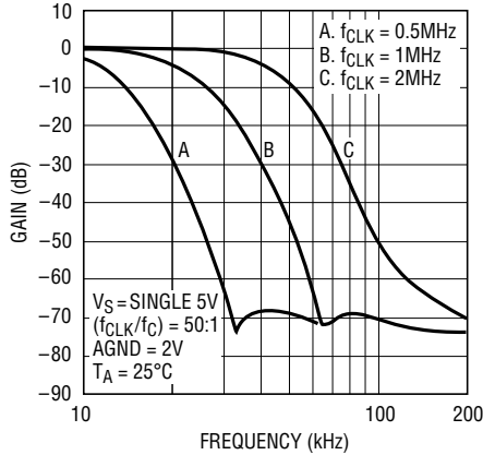
Gain vs f_{CLK}
