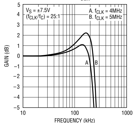
Passband Gain vs f_{CLK} at 85^\circ C
