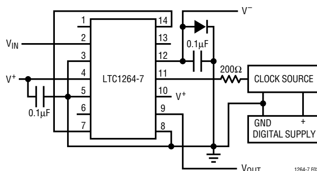
Figure 2. Dual Supply Operation for an f_{\text{CLK}}/f_{\text{CUTOFF}} = 25:1
