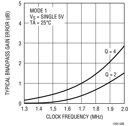
Typical Bandpass Gain Error vs Clock Frequency
