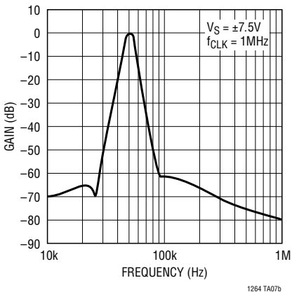
50kHz Bandpass Filter, Linear Phase Gain vs Frequency
