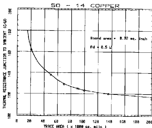
Figure 7 : R_{th(j-a)} of SO-14 vs. on Board Trace Area.
