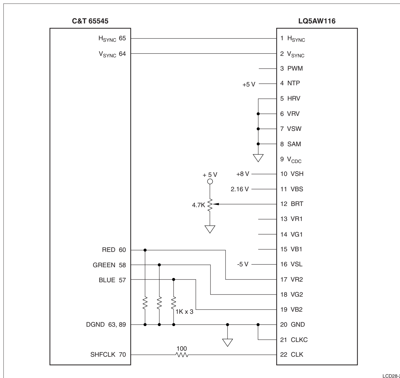
Figure 2. System Wiring Diagram
