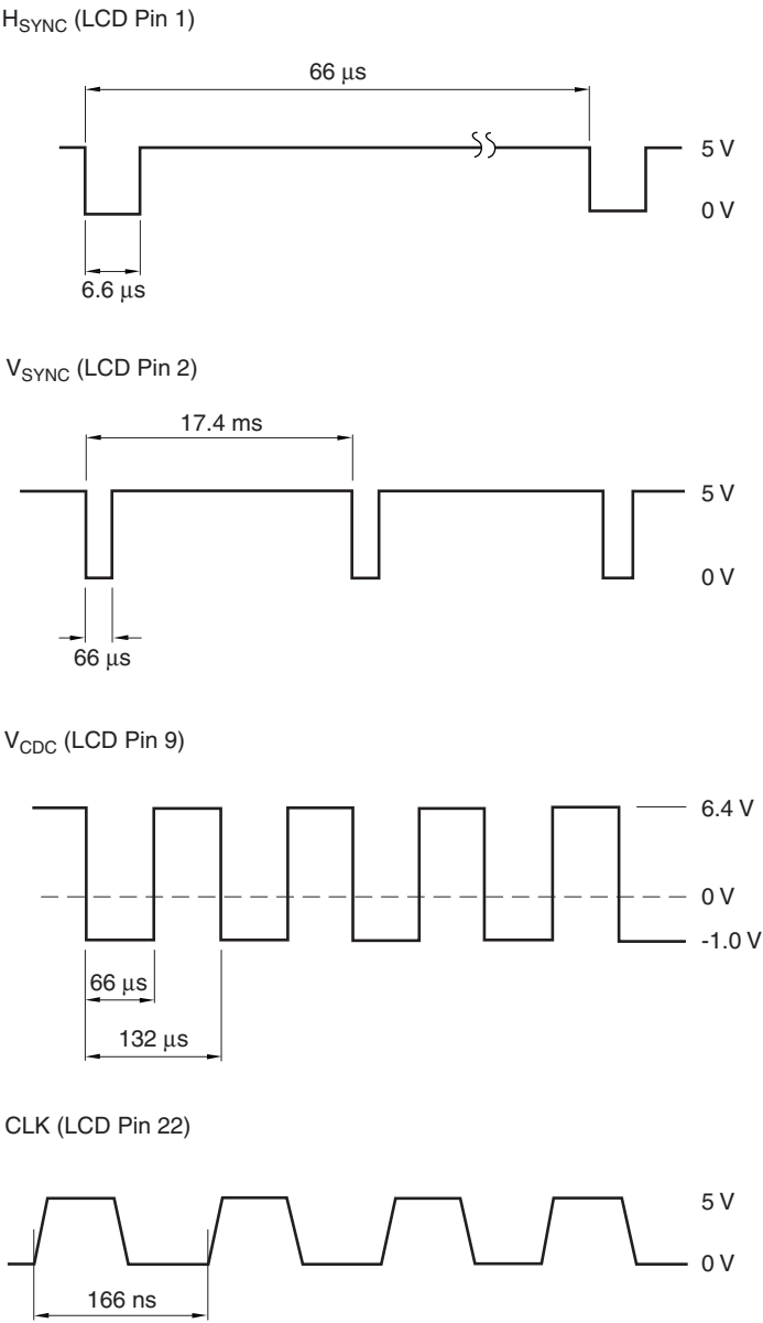
Figure 3. LQ5AW116 Timing Diagrams
