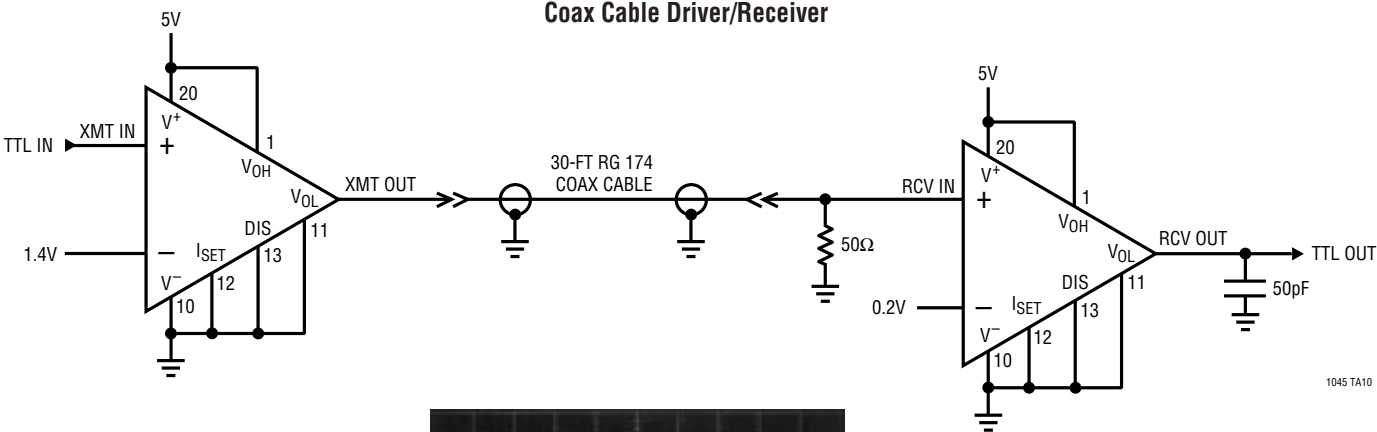
Coax Cable Driver/Receiver
