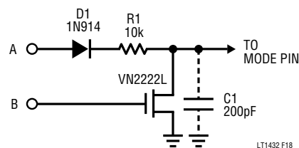
Figure 18. Two Input Mode Drive
