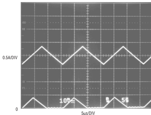
Figure 10. Inductor Current
