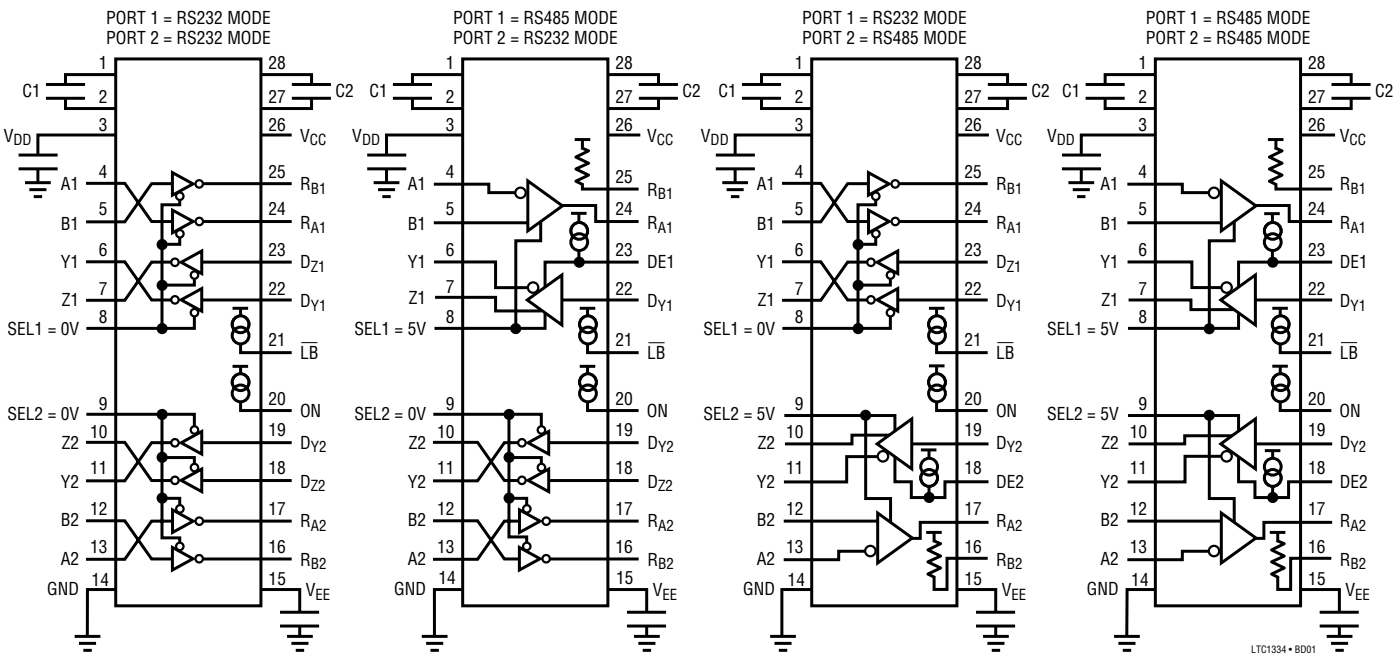
Interface Configuration with Loopback Disabled
