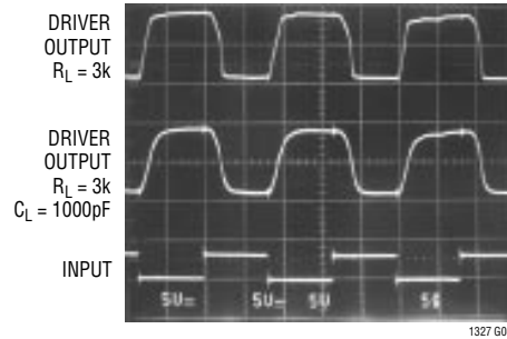
Driver Output Waveform
