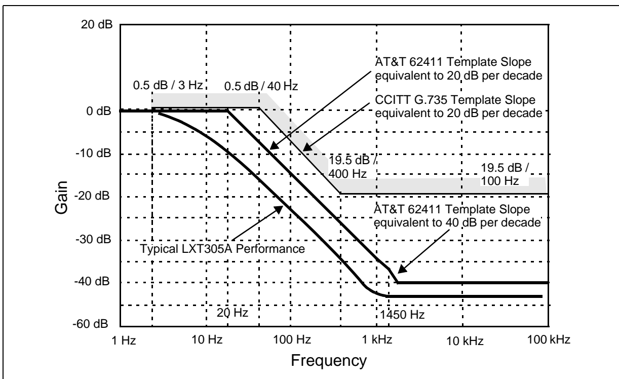
Figure 8. LXT305A Transmit Jitter Transfer Performance (Typical)
