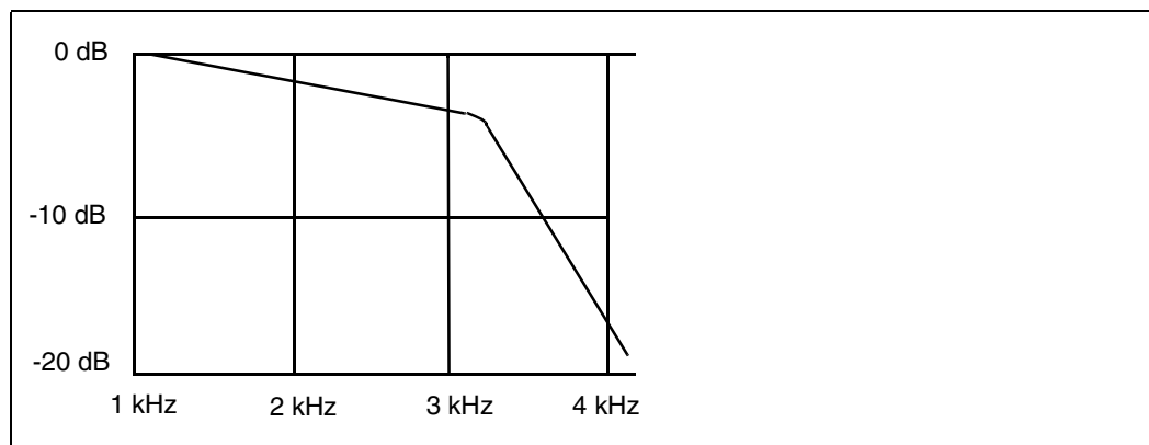
Figure 3. C-Message Weighting
