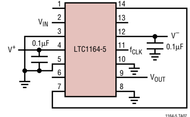
8th Order Linear Phase Lowpass Filter f_{CLK}/f_C = 140:1
