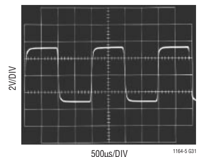
Transient Response V_{IN} = \pm 3\text{V} , 500Hz Square Wave
