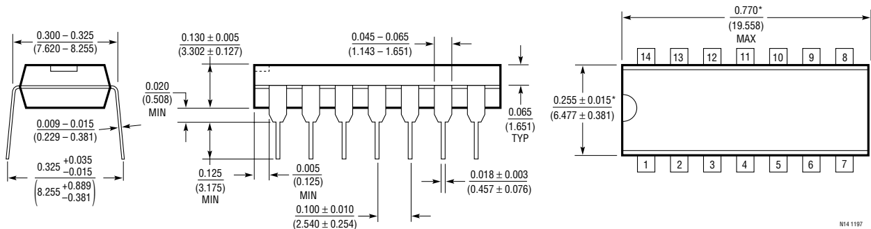
N Package 14-Lead PDIP (Narrow 0.300) (LTC DWG # 05-08-1510)
