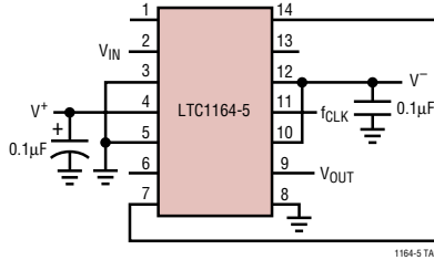
8th Order Butterworth Lowpass Filter f_{CLK}/f_C = 100:1
