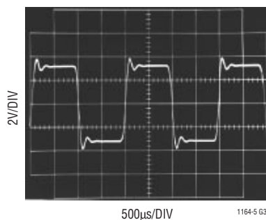
Transient Response V_{IN} = \pm 3\text{V} , 500Hz Square Wave
