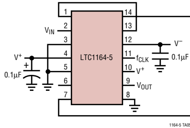
8th Order Butterworth Lowpass Filter f_{CLK}/f_C = 50:1
