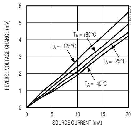
REVERSE VOLTAGE vs. CURRENT
