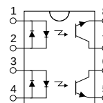
LDA200 Pinout
