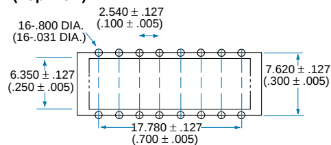
PC Board Pattern (Top View)
