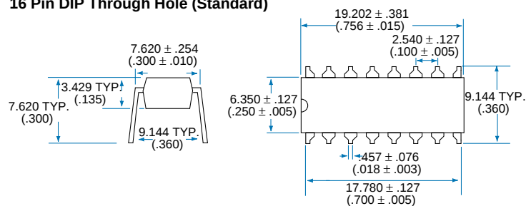
16 Pin DIP Through Hole (Standard)
