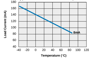
LCC110 - FormB Typical Load Current vs. Temperature
