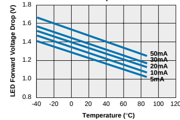
LCC110 Typical LED Forward Voltage Drop vs. Temperature
