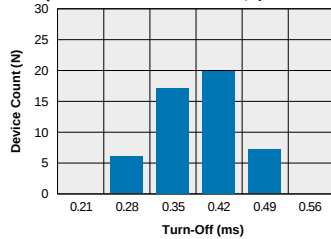
LCC110 - FormB Typical Turn-Off Time (N=50 Ambient Temperature = 25°C) (Load Current = 120mADC; I_F = 8\text{mADC} )
