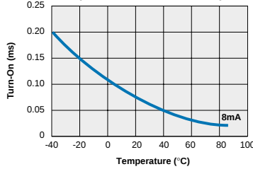
LCC110 - FormB Typical Turn-On vs. Temperature (Load Current = 120mADC)
