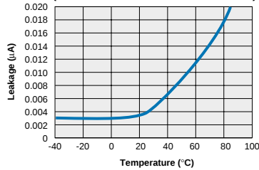
LCC110 Typical Leakage vs. Temperature (Measured across Pins 5 & 6 or 7 & 8)
