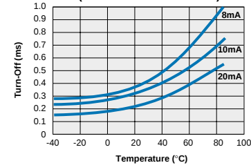
LCC110 - FormB Typical Turn-Off vs. Temperature (Load Current = 120mADC)
