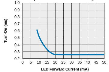
LCC110 - FormA Typical Turn-On vs. LED Forward Current (Load Current = 120mADC)
