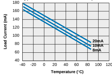
LCC110 - FormA Typical Load Current vs. Temperature
