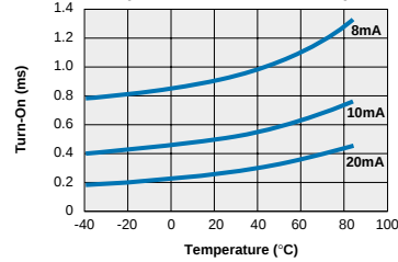
LCC110 - FormA Typical Turn-On vs. Temperature (Load Current = 120mADC)
