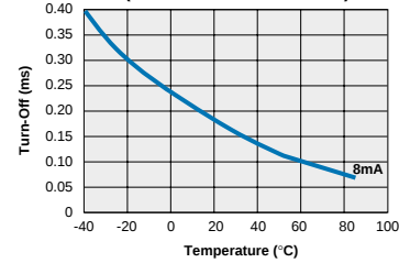
LCC110 - FormA Typical Turn-Off vs. Temperature (Load Current = 120mADC)
