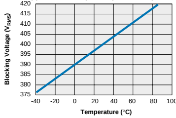
LCC110 - FormA Typical Blocking Voltage vs. Temperature
