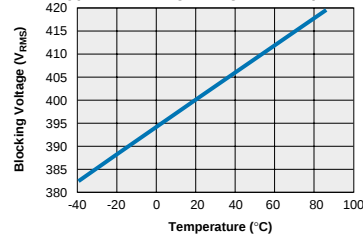
LCC110 - FormB Typical Blocking Voltage vs. Temperature
