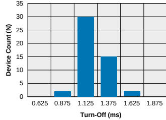
LBA120L - Form B Typical Turn-Off Time (N=50 Ambient Temperature = 25°C) (Load Current = 170mADC; I_F = 5\text{mADC} )
