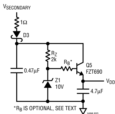
Figure 2. V_{DD} Regulator
