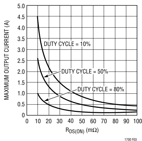
Figure 3. Maximum Current vs R_{DS(ON)}
