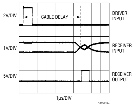
Figure 14a. 4000ft of Category 5 UTP: 1μs Pulse
