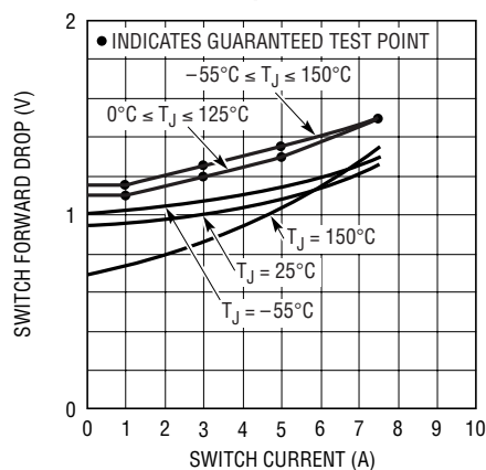
LT1089 Switch Voltage vs Output Current
