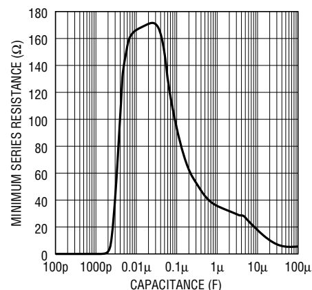
Output Minimum Series Resistance vs Load Capacitance
