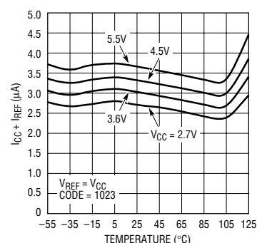
Total Supply-Plus-Reference Operating Current
