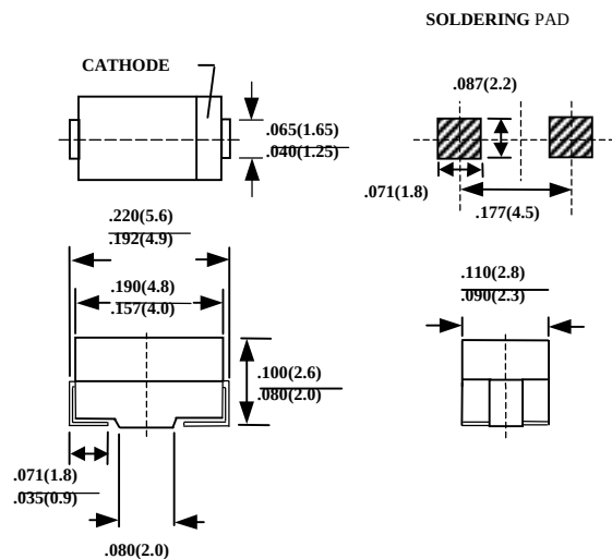
CASE : SMA ( DO-214AC) DIMENSIONS IN INCHES AND (MILLIMETERS)
