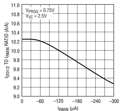
I_{DI01/2} to I_{RMIN} Ratio vs R_{MIN} Current
