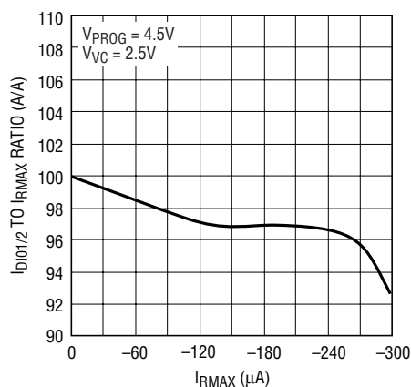
I_{DI01/2} to I_{RMAX} Ratio vs R_{MAX} Current
