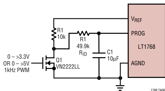
PWM Intensity Control From 3.3V or 5V Logic
