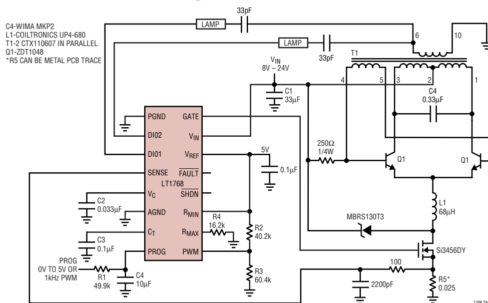
Figure 1. 14W CCFL Supply Produces a 100:1 Dimming Ratio While Maintaining Minimum and Maximum Lamp Current Specifications
