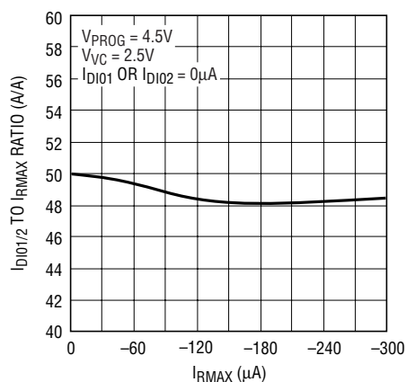
I_{DI01/2} to I_{RMAX} Ratio vs R_{MAX} Current with a Lamp Fault
