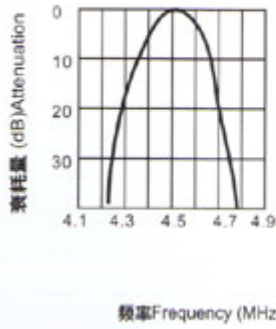
LT4.5MB频率特性 LT4.5MB Frequency Characteristics
