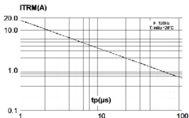
Figure 2. Repetitive peak pulse current versus pulse duration (maximum values)
