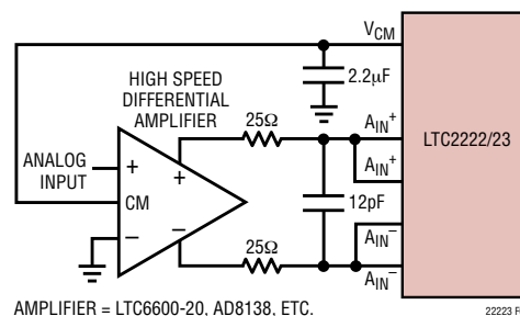
Figure 4. Differential Drive with an Amplifier
