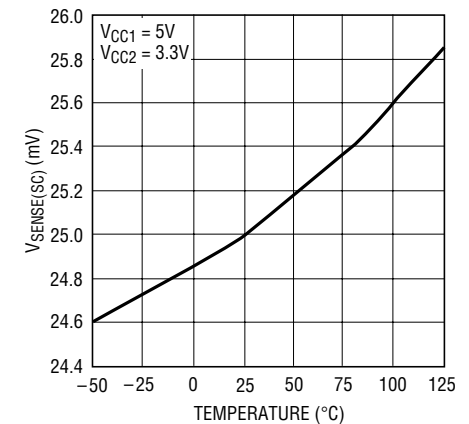
V_{\text{SENSE(SC)}} vs Temperature
