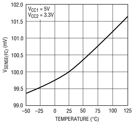
V_{\text{SENSE(FC)}} vs Temperature
