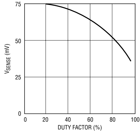
Maximum Current Sense Threshold vs Duty Factor
