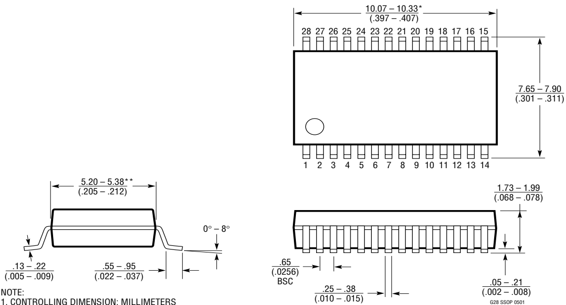
G Package 28-Lead Plastic SSOP (5.3mm) (Reference LTC DWG # 05-08-1640)
