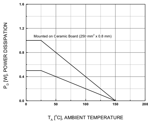
Figure 5. Power Derating
