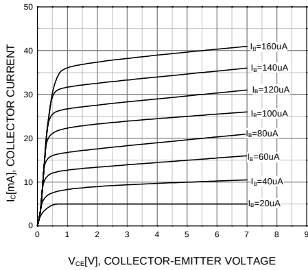
Figure 1. Static Characteristic
