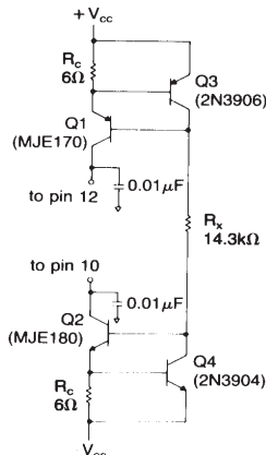
Figure 4: Active current limit circuit (100mA)
