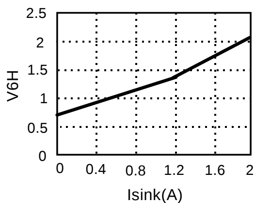
Figure 3. Isink-V6H
