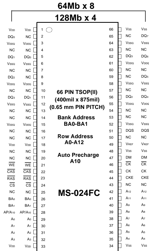
Figure 1. 256Mb package Pinout
