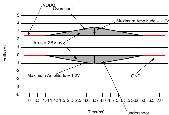
Figure 25. AC overshoot/Undershoot Definition
