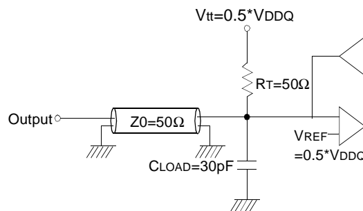
Figure 26. Output Load Circuit (SSTL_2)
