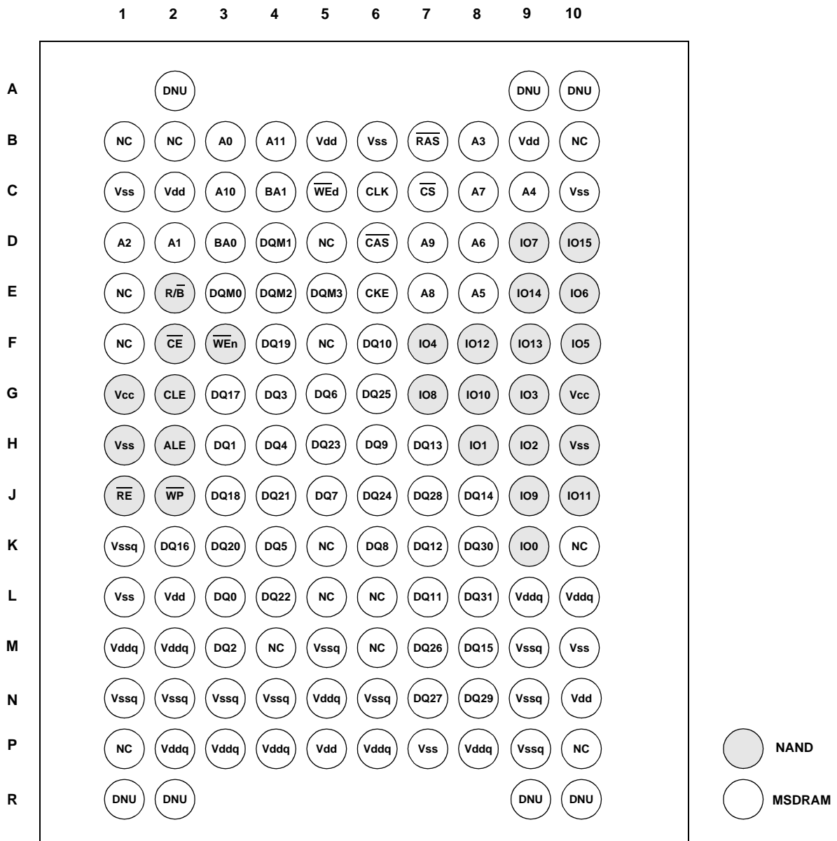
137 FBGA: Top View (Ball Down)
