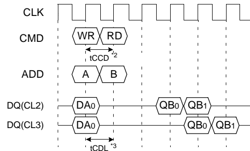
3) Write interrupted by Read (BL=2)
