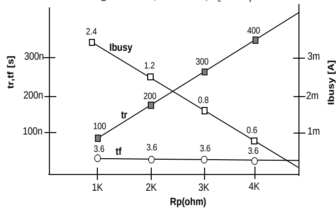
Fig 17 R_p vs t_r, t_f & R_p vs i_{\text{busy}}
