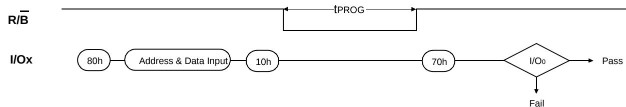
Figure 8. Program Operation
