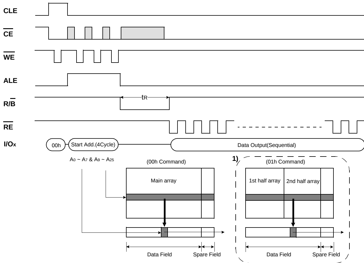
Figure 6. Read1 Operation
