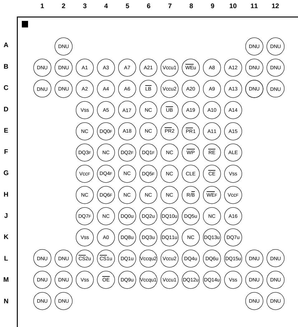
111-TBGA: Top View (Ball Down)
