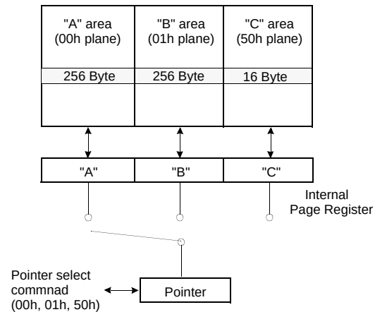
Figure 16. Block Diagram of Pointer Operation
