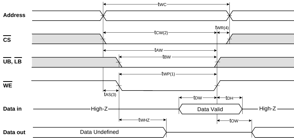
TIMING WAVEFORM OF WRITE CYCLE(1) ( \overline{WE} Controlled, \overline{PR}=V_{IH} )
