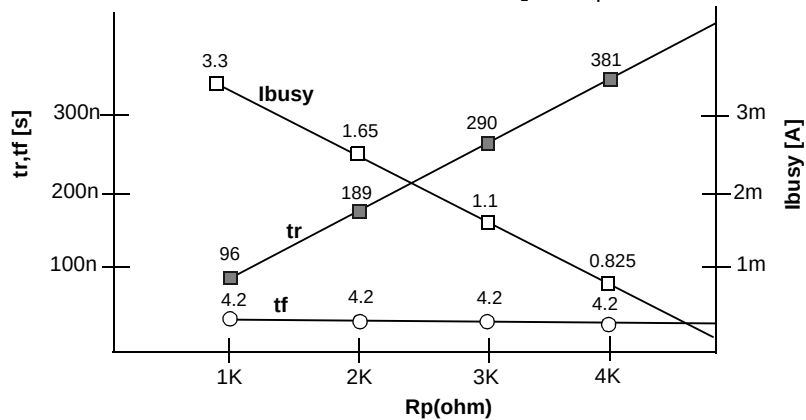
Figure 9. R_p vs t_r, t_f & R_p vs i_{busy}
