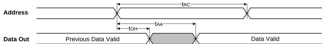
TIMING WAVEFORM OF READ CYCLE(1) (Address Controlled, \overline{CS}=\overline{OE}=V_{IL} , \overline{PR}=\overline{WE}=V_{IH} , \overline{UB} or/and \overline{LB}=V_{IL} )
