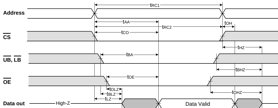
TIMING WAVEFORM OF READ CYCLE(2) ( \overline{PR}=\overline{WE}=V_{IH} )
