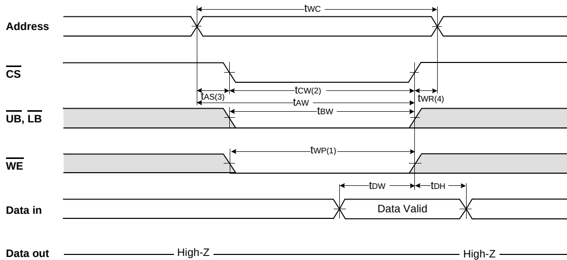
TIMING WAVEFORM OF WRITE CYCLE(2) ( \overline{CS} Controlled, \overline{PR}=V_{IH} )
