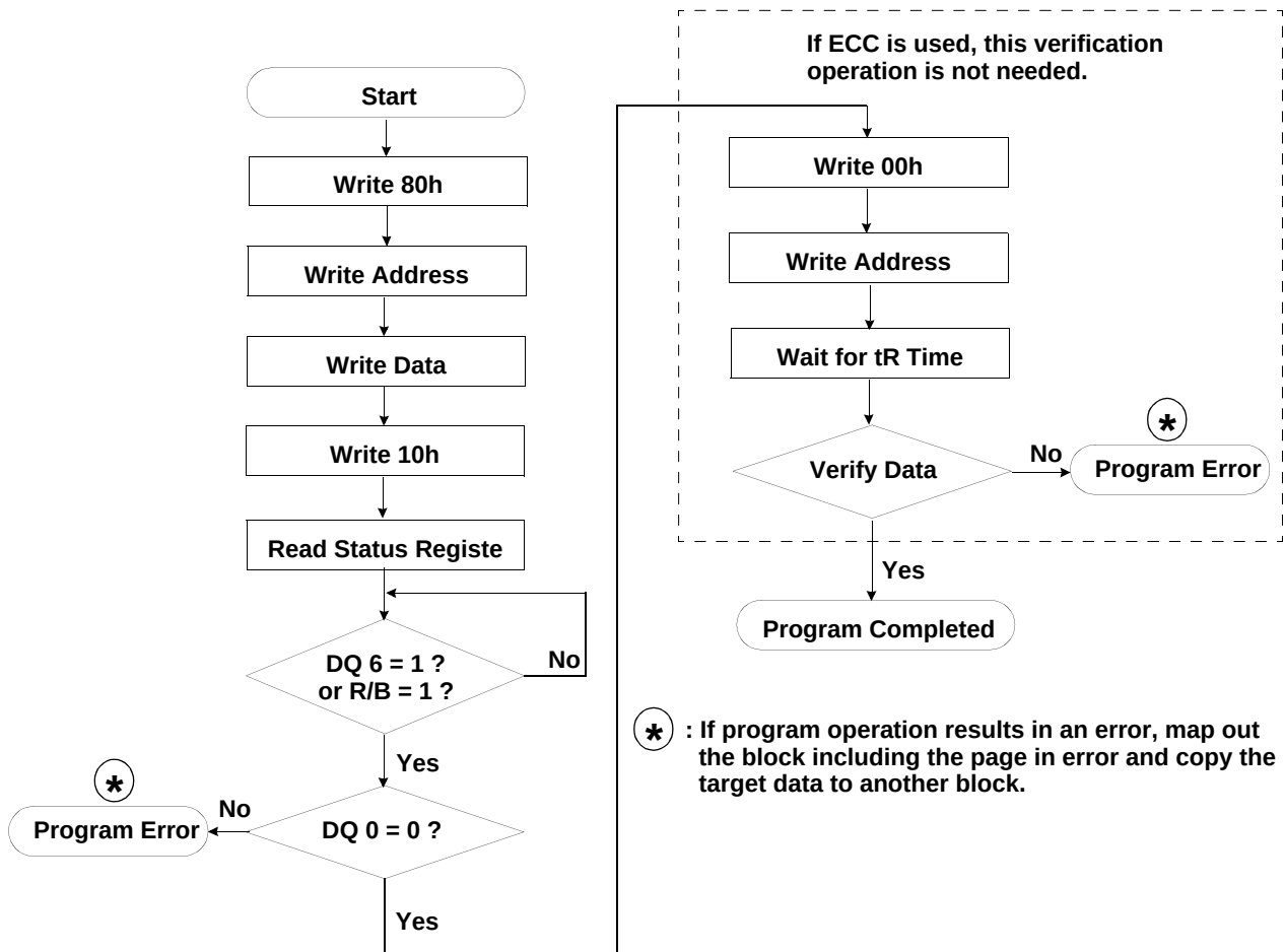
Figure 12. Flash Program flow chart
