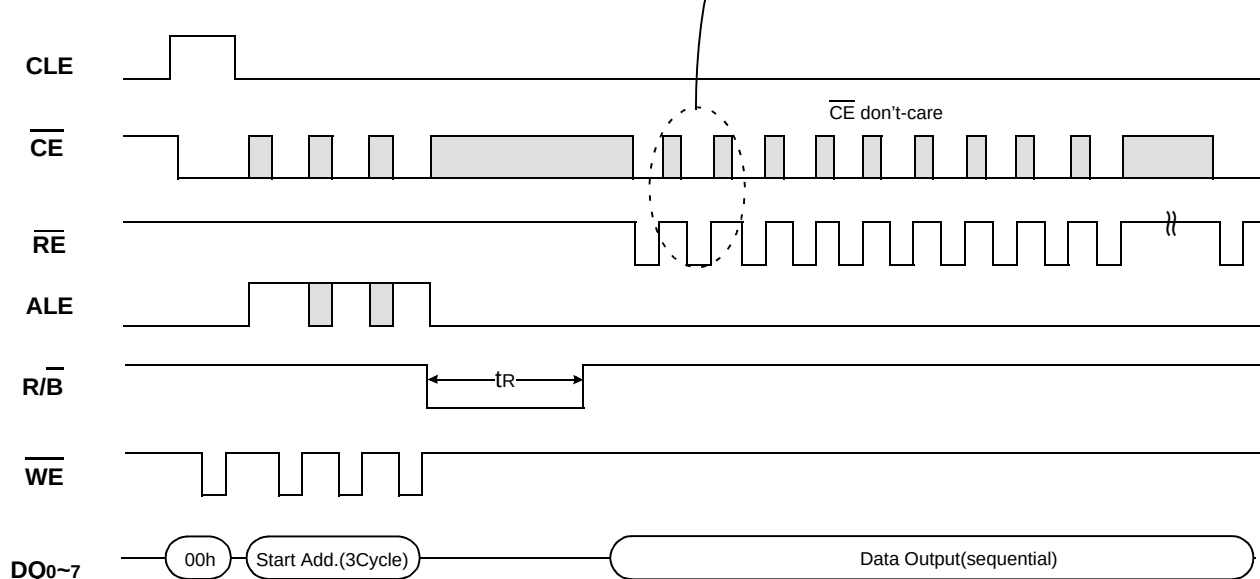
Figure 18. Read Operation with \overline{\text{CE}} don't-care.
