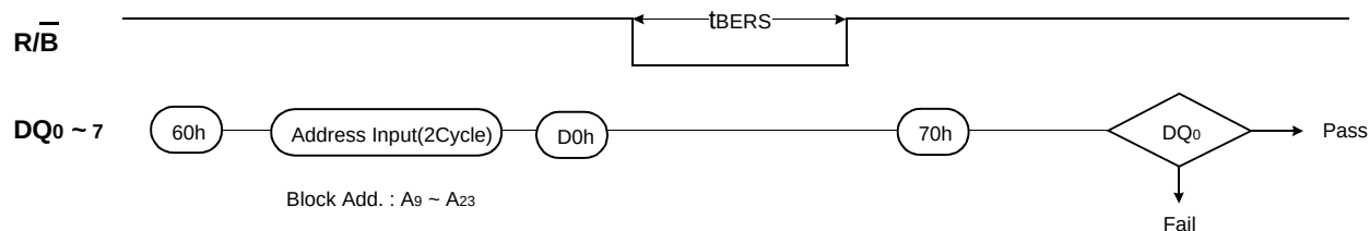
Figure 6. Block Erase Operation
