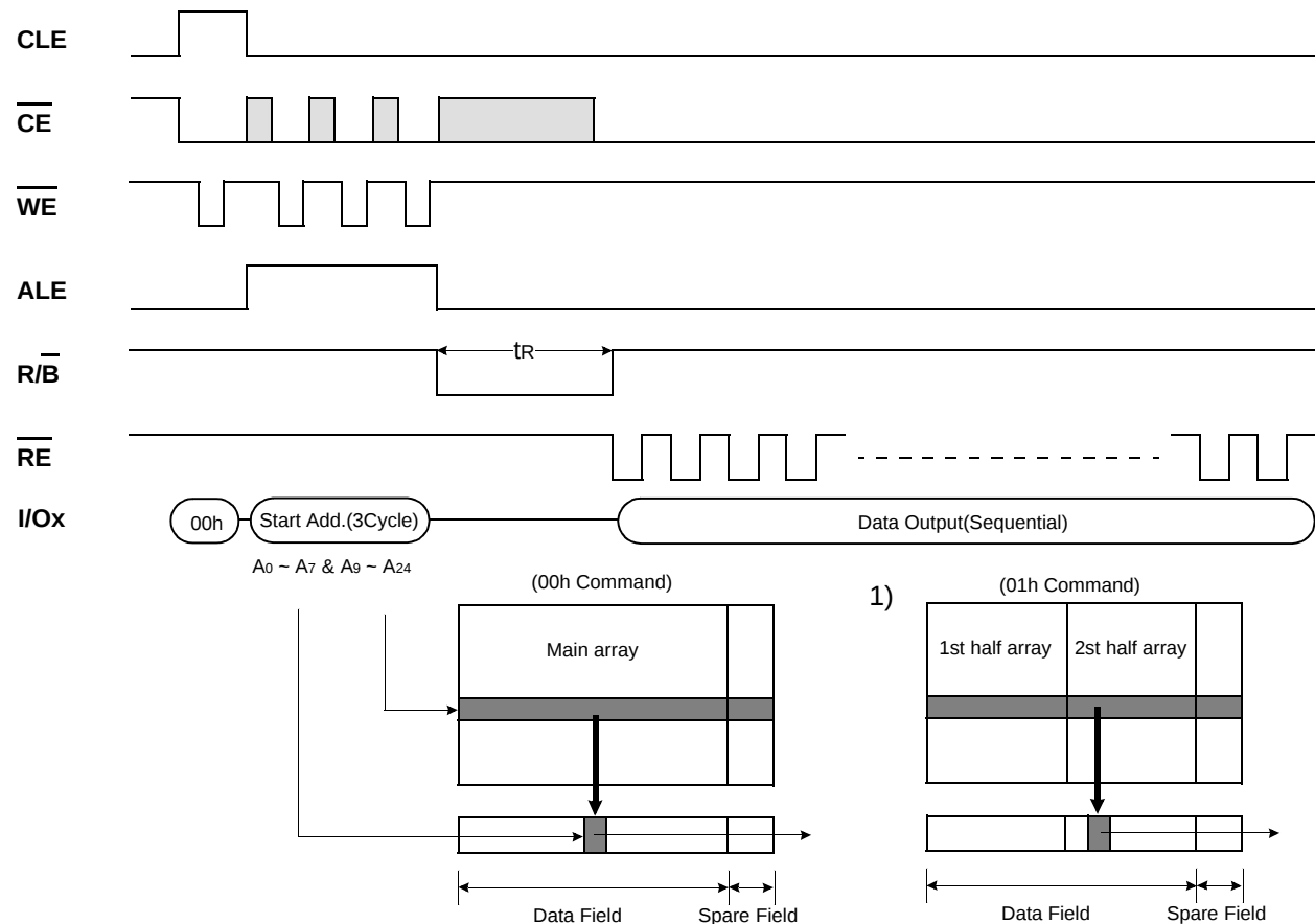
Figure 6. Read1 Operation
