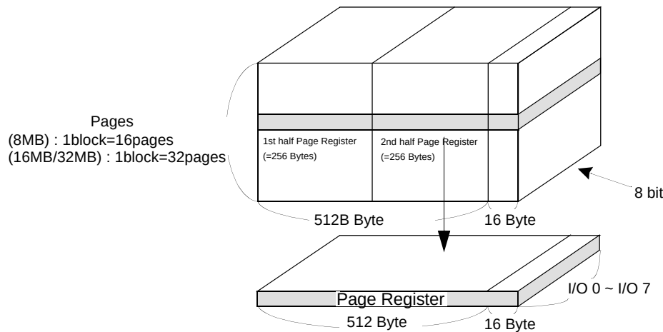
Figure 2. ARRAY ORGANIZATION
