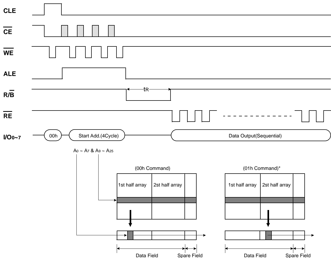
Figure 8. Read1 Operation
