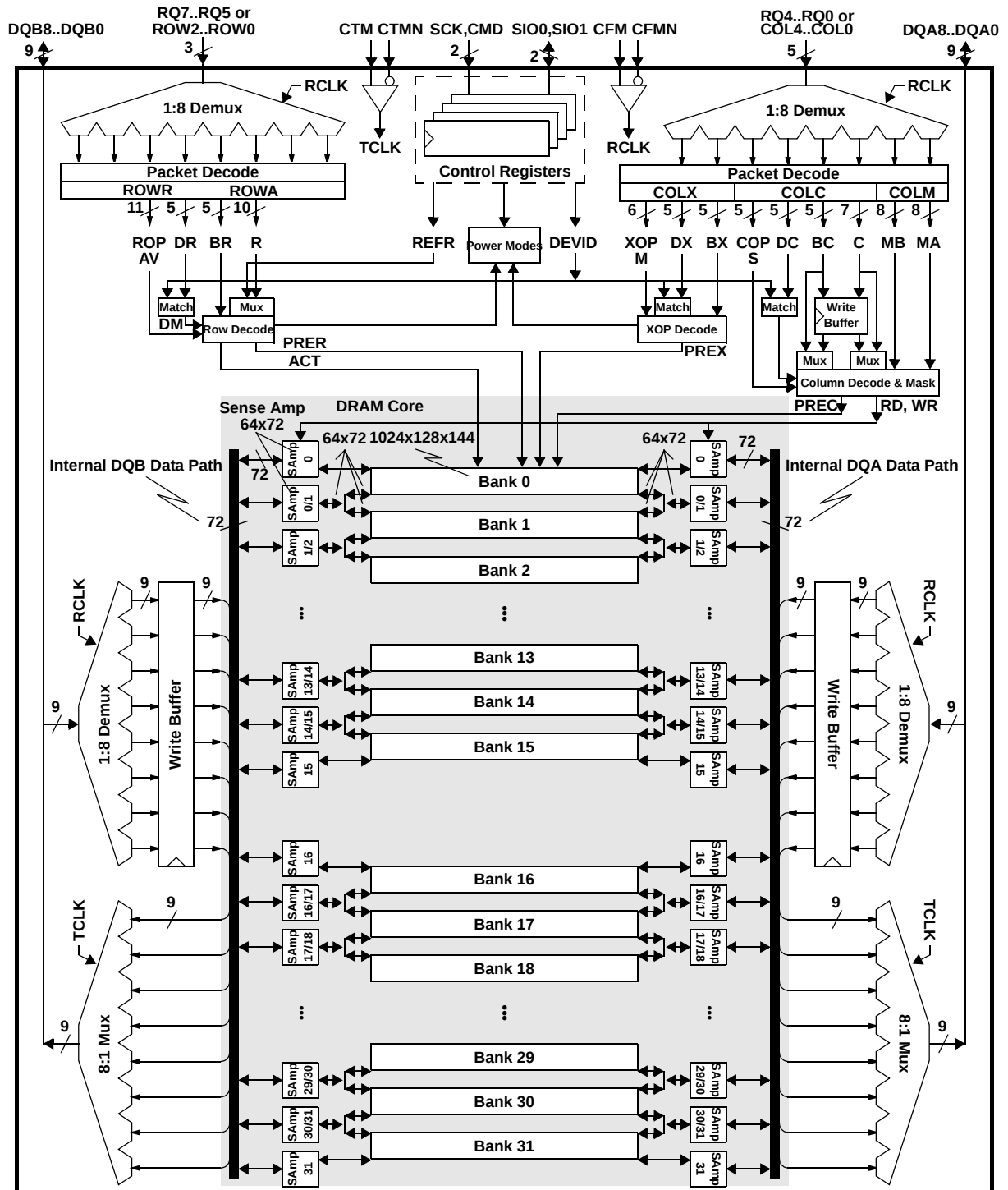
Figure 2: 576Mbit (1M x18 x32s) RDRAM Device Block Diagram
