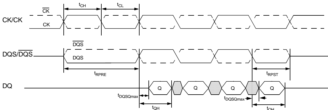
&lt;Data output (read) timing&gt;
