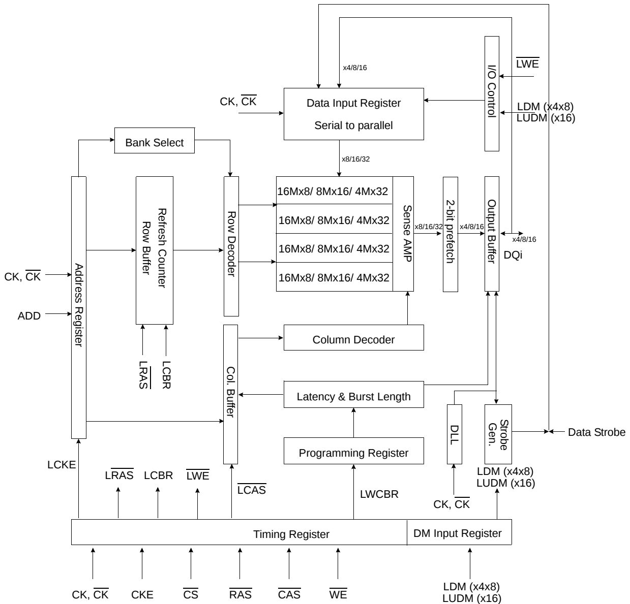
Block Diagram (32Mb x 4 / 16Mb x 8 / 8Mb x 16 I/O x 4 Banks)
